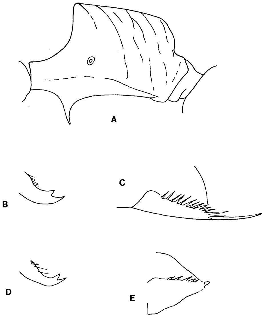
Fig. 1. Recent and fossil Paraponera ant workers. P. clavata , the living species, anatomical features of a worker from Isla Paloma, Orinoco Delta, Venezuela: A, left side of petiole; B, claw of fore tarsus; C, left side of terminal segment of gaster, showing sting and comb of spinules fringing the hypopygidial border. Paraponera sp. from the Dominican amber: D, claw of fore tarsus; E, left side of terminal segment of gaster.
