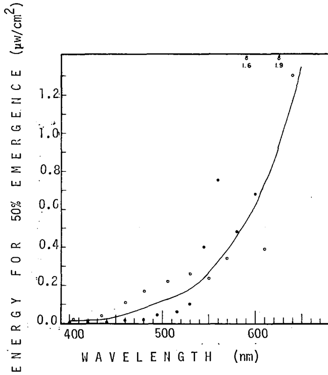
Fig. 3.--Action spectrum for breaking diapause in oak silkworm pupae. Solid circles are data from Expt 1 with a single filter spectrograph (20-25 nm bandpass). Open circles are data from Expt 2 with a double filter spectrograph (10-13 nm bandpass). The curve represents the best estimate of the spectrum from the combined experiments. (From Norris et al. , 1969).
