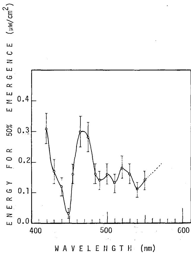
Fig. 4.--Action spectrum for breaking diapause in codling moth larvae. The error bars show the estimated uncertainty at each point. (From Norris et al. , 1969).
