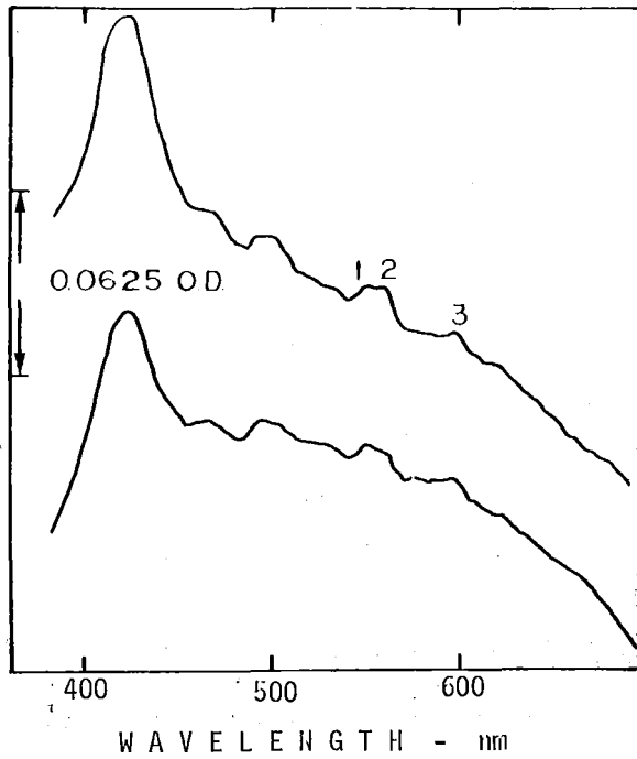
Fig. 6.--Absorption spectrum of 70 codling moth brains after reduction with sodium dithionite and cooling to liquid N 2 temperature. The 2 curves represent different orientations of the same sample in the light path. O.D. = optical density.
