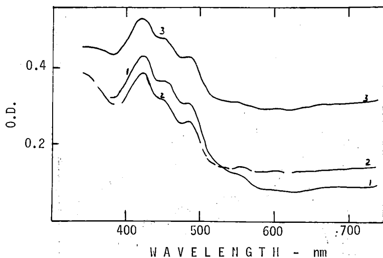
Fig. 5.--Absorption spectrum obtained from 26 intact oak silkworm brains. 1. As isolated from insects, after storage at -178^{\circ}\text{C} for 48 hr. 2. Brains 5 min. after treatment with sodium dithionite solution. 3. Curve 10 min after treatment with sodium dithionite solution. O.D. = optical density.
