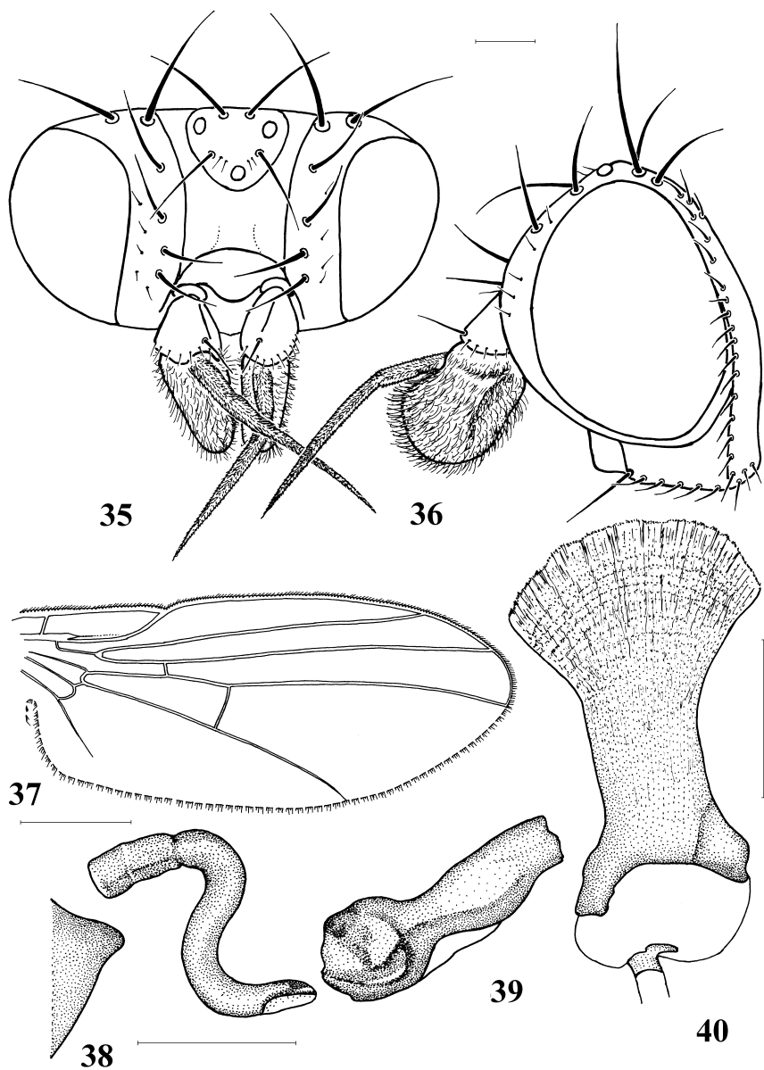
Figs. 35–40. Cerodontha (Dizygomyza) crassiseti . 35. Head, frontal view. 36. Head, lateral view. 37. Wings. 38. Caudal projection, lateral view. 39. Phallus, lateral view. 40. Ejaculatory apodeme, lateral view. Scale bars = 0.1 mm, except for Fig. 37 = 0.5 mm (Figs. 39 and 40, after Nowakowski, 1973).
